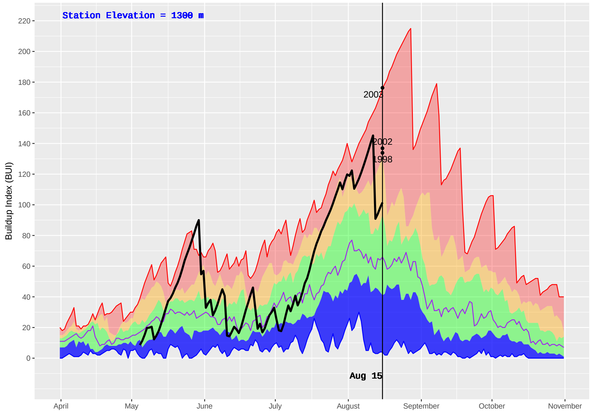
MARION (367) : Historical (1994–2016) and Current (2018) Daily Buildup Index (BUI)
