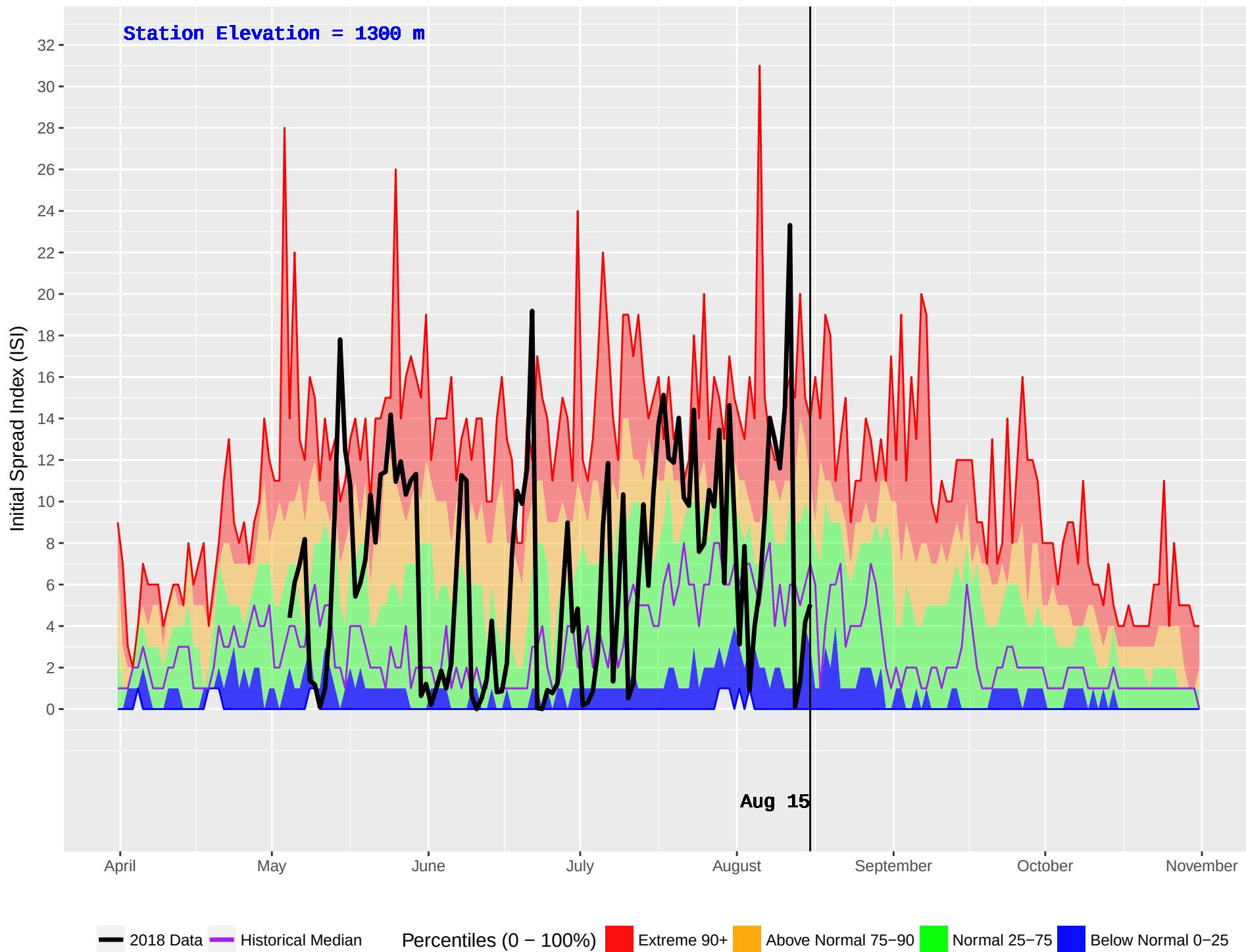
MARION (367) : Historical (1994–2016) and Current (2018) Daily Initial Spread Index (ISI)
