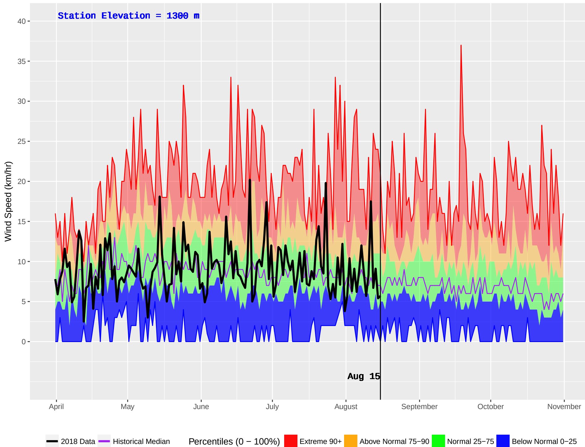
MARION (367) : Historical (1994–2016) and Current (2018) Daily Wind Speed
