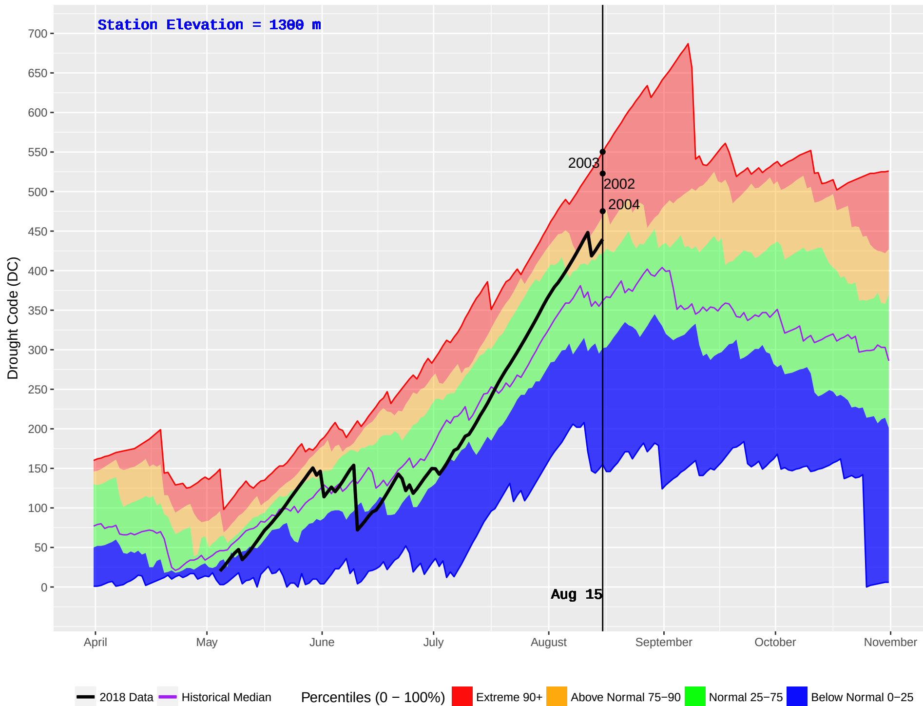
MARION (367) : Historical (1994–2016) and Current (2018) Daily Drought Code (DC)
