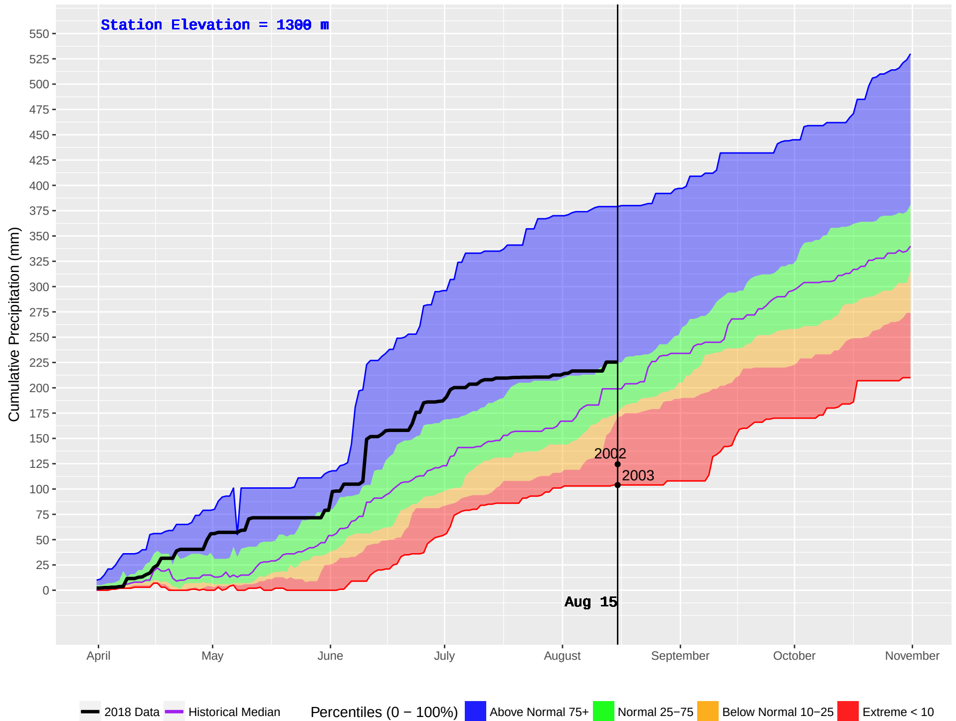
MARION (367) : Historical (1994–2016) and Current (2018) Daily Cumulative Precipitation
