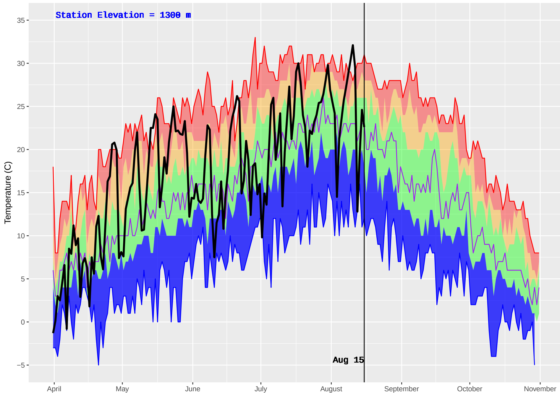
MARION (367) : Historical (1994–2016) and Current (2018) Daily Temperature
