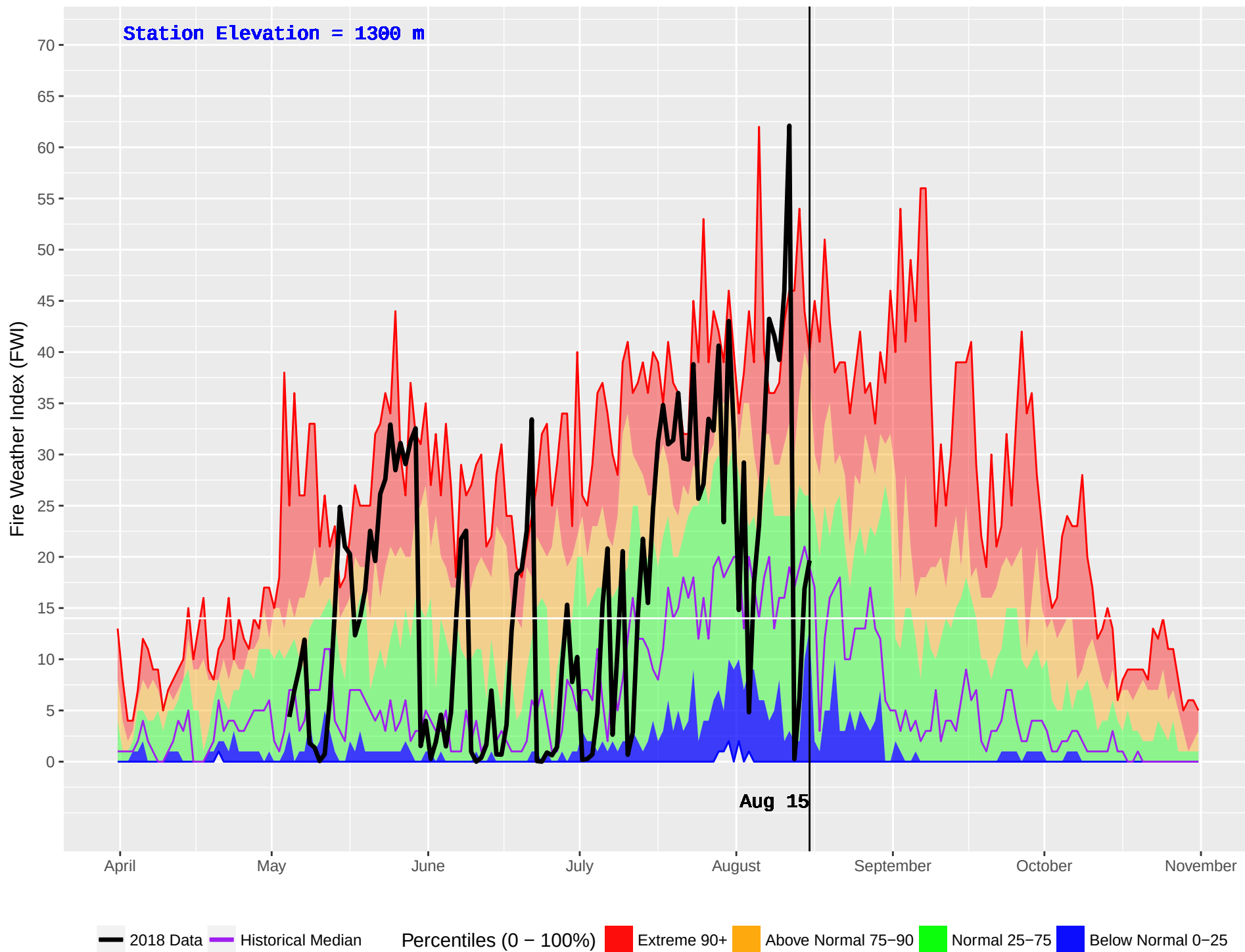
MARION (367) : Historical (1994–2016) and Current (2018) Daily Fire Weather Index (FWI)
